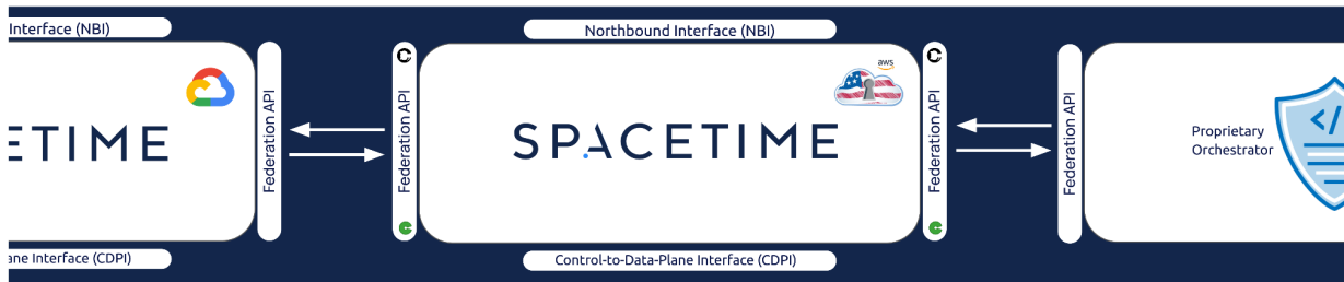
Figure 5: Federation API
