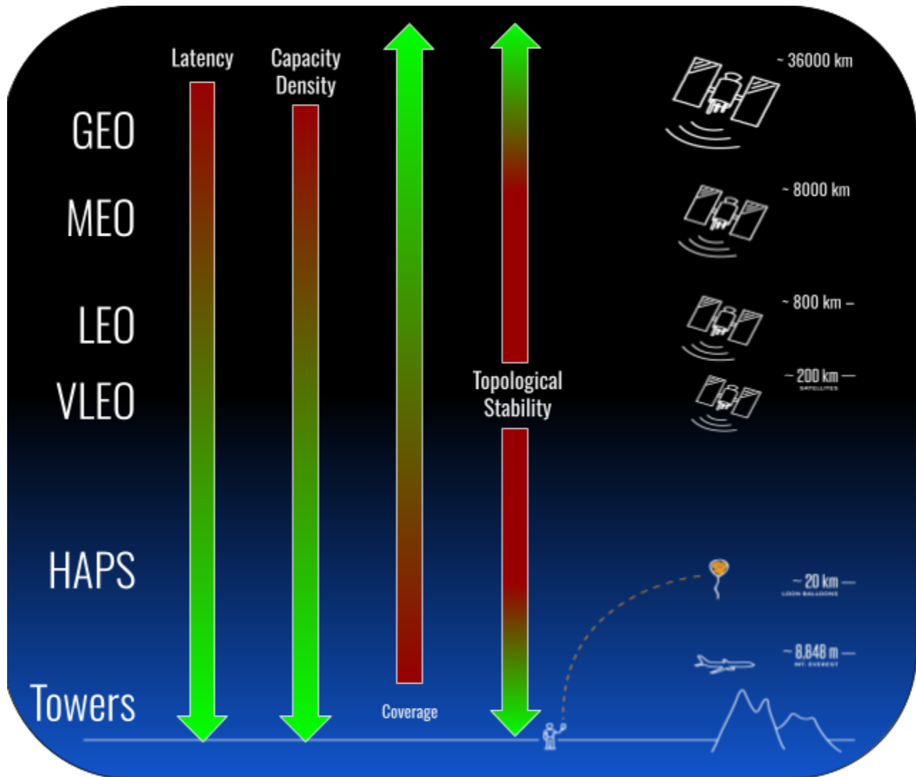
Figure 1: Characteristics of different orbital regimes and domains
